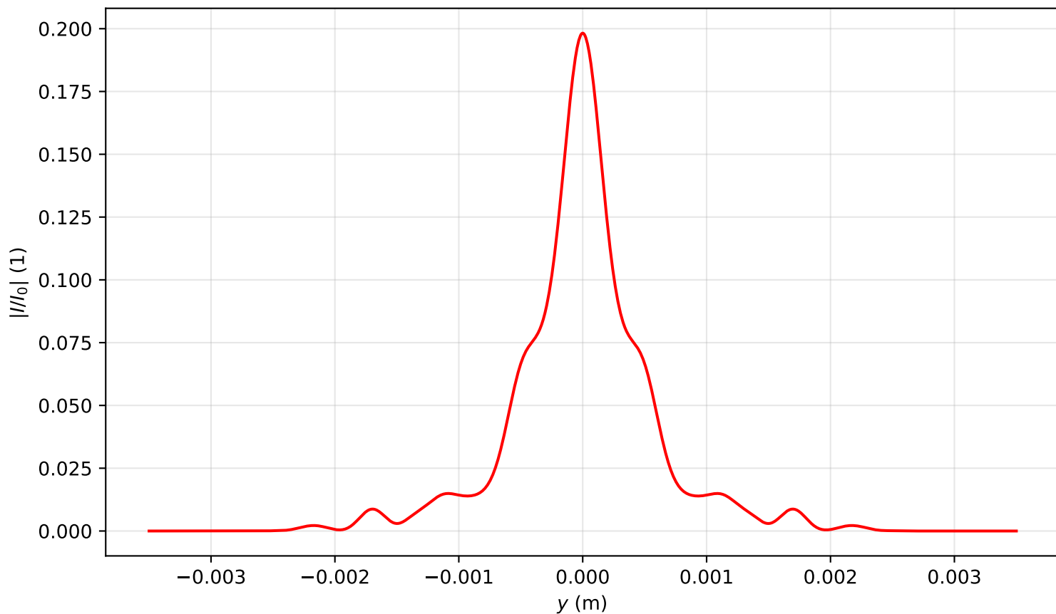
Intensity profile I(x=0, y, z=3.821)/I_0 , \text{Pin}=5.0\text{Pcr} , artificial time
